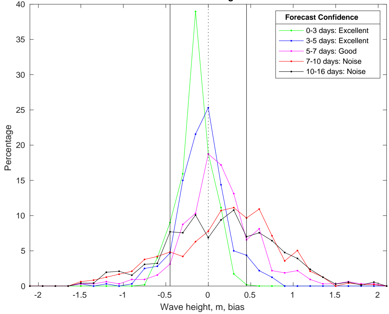
NDBC 42035 vs GFSWaves Bias Histogram: 02-Feb-2025
