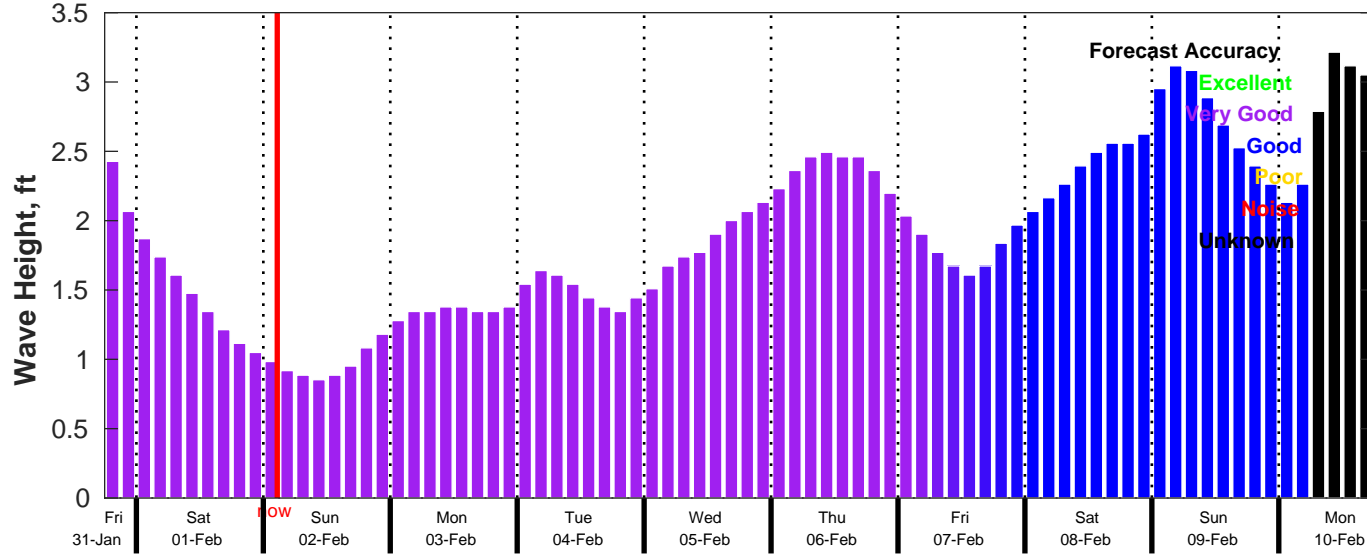
CMEMS Wave Forecast for NDBC 42035 from 31-Jan-2025 18:00:00 to 10-Feb-2025 18:00:00
