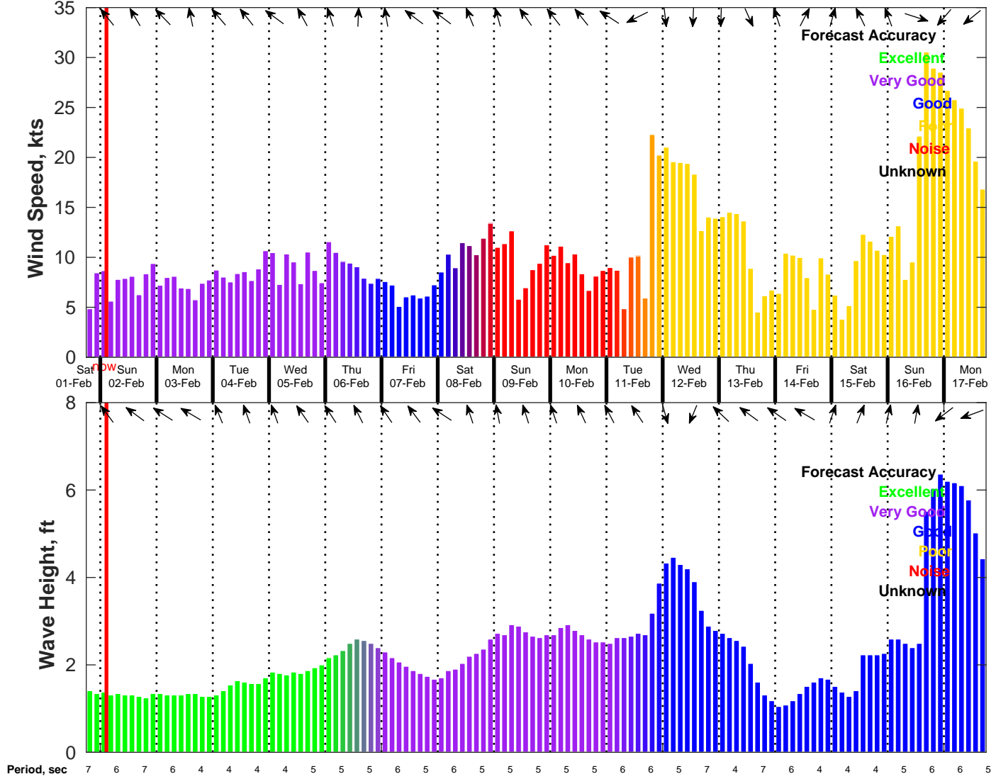
Wind & Wave Forecast for NDBC 42035 from 01-Feb-2025 18:00:00 to 17-Feb-2025 18:00:00
