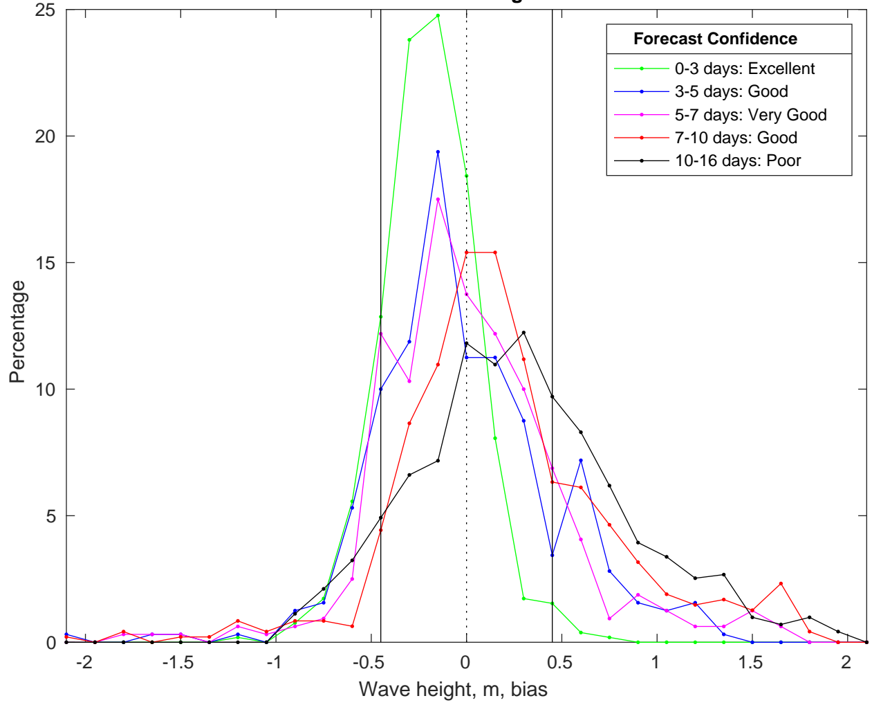
NDBC 42036 vs GFSWaves Bias Histogram: 02-Feb-2025
