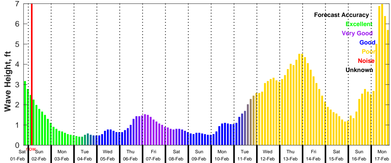
GFS Wave Forecast for NDBC 42036 from 01-Feb-2025 19:00:00 to 17-Feb-2025 19:00:00
