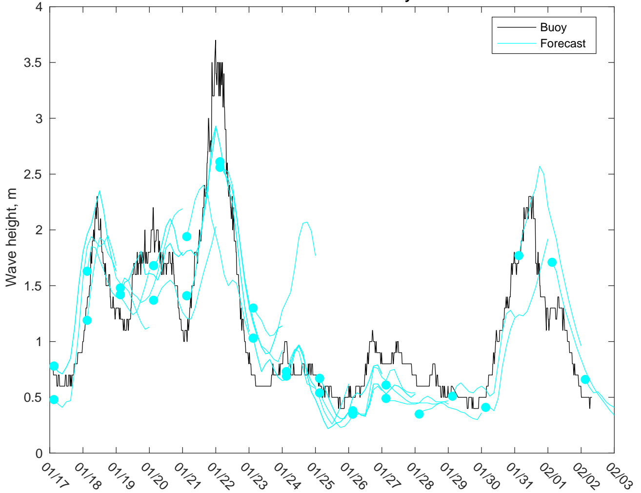
NDBC 42040 vs CMEMSWaves: 5 to 7 day forecast
