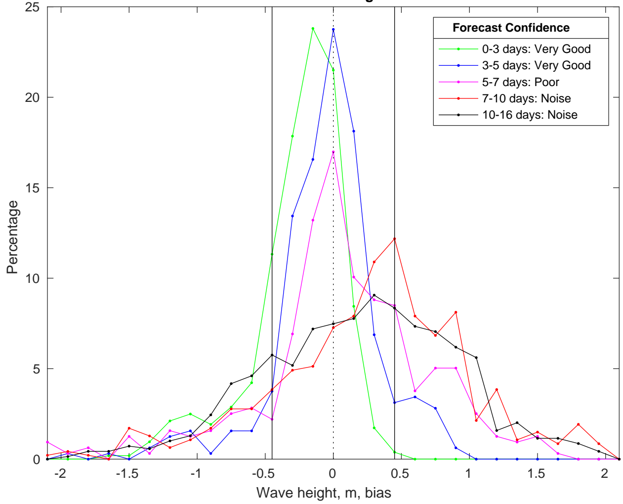
NDBC 42040 vs GFSWaves Bias Histogram: 02-Feb-2025
