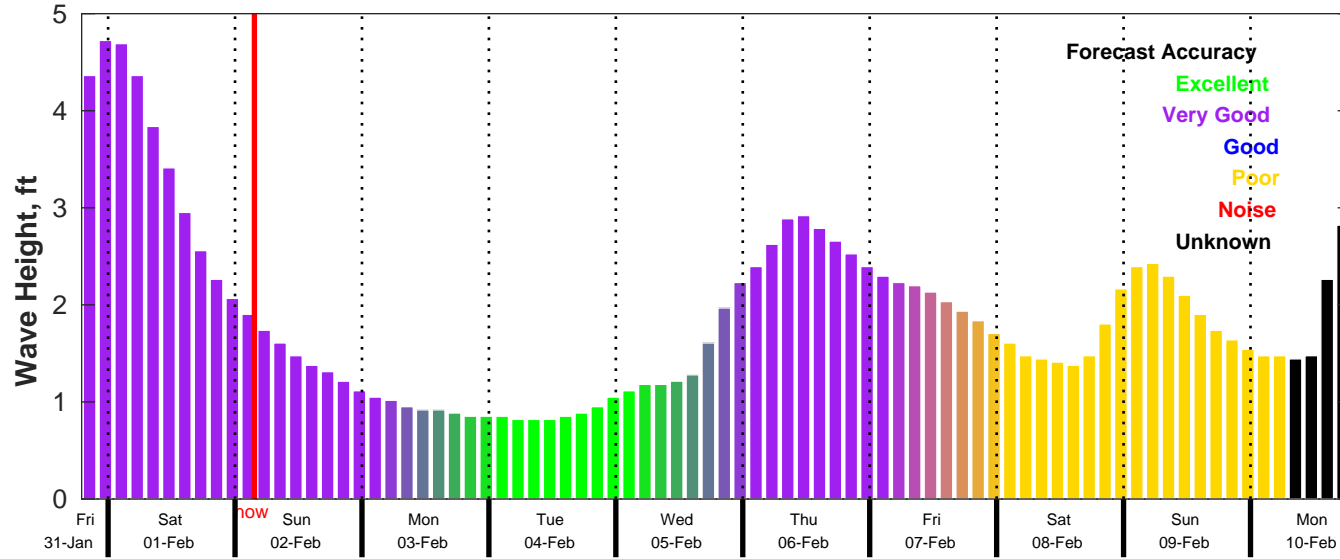
CMEMS Wave Forecast for NDBC 42040 from 31-Jan-2025 19:00:00 to 10-Feb-2025 19:00:00
