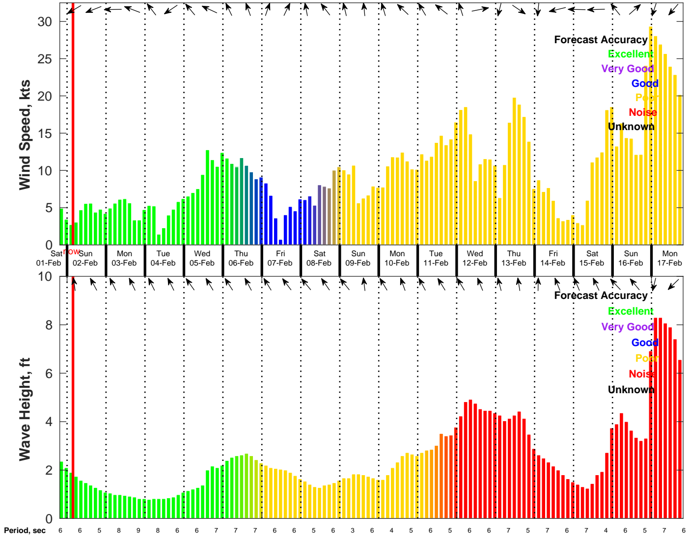
Wind & Wave Forecast for NDBC 42040 from 01-Feb-2025 19:00:00 to 17-Feb-2025 19:00:00
