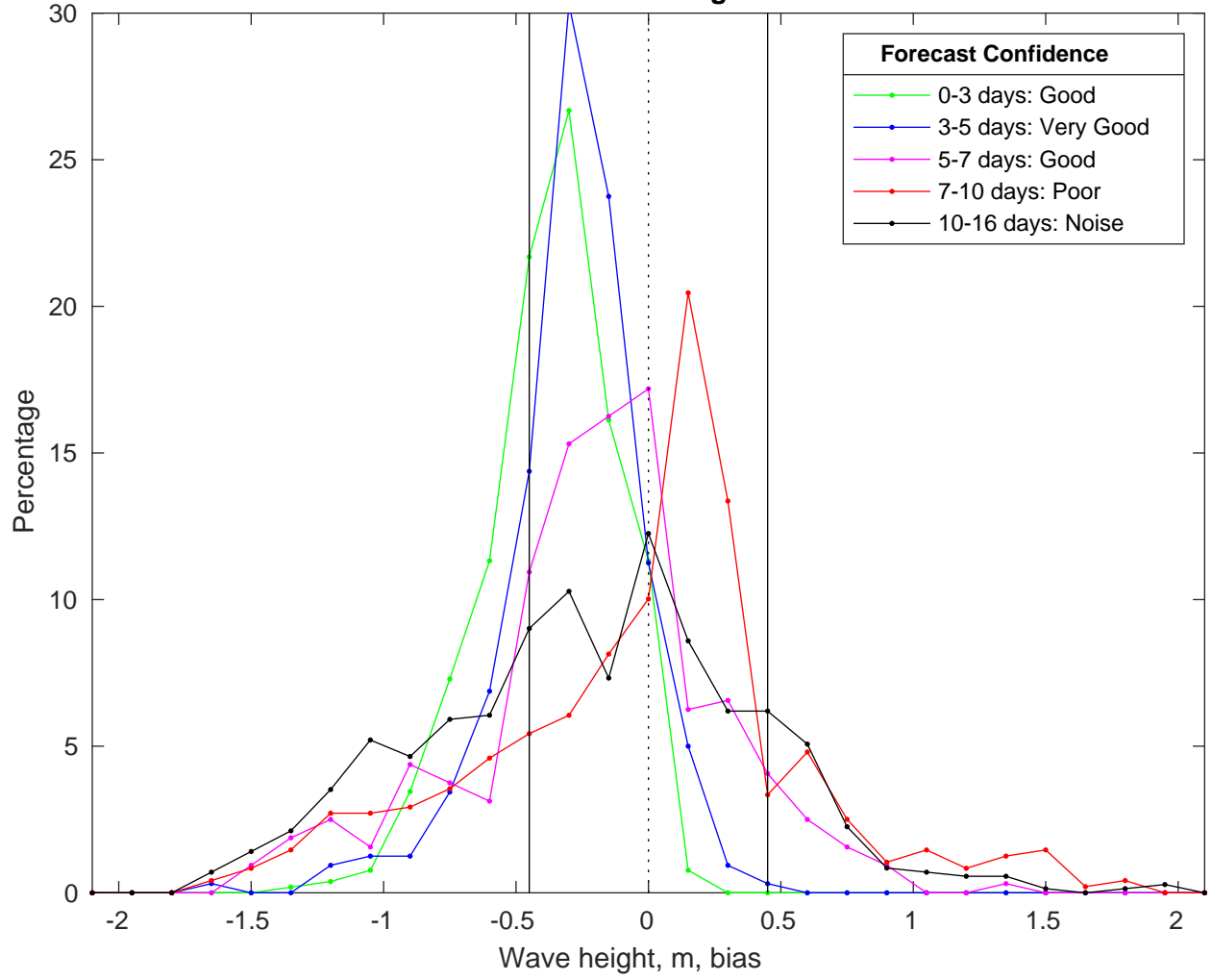
NDBC 42084 vs GFSWaves Bias Histogram: 02-Feb-2025
