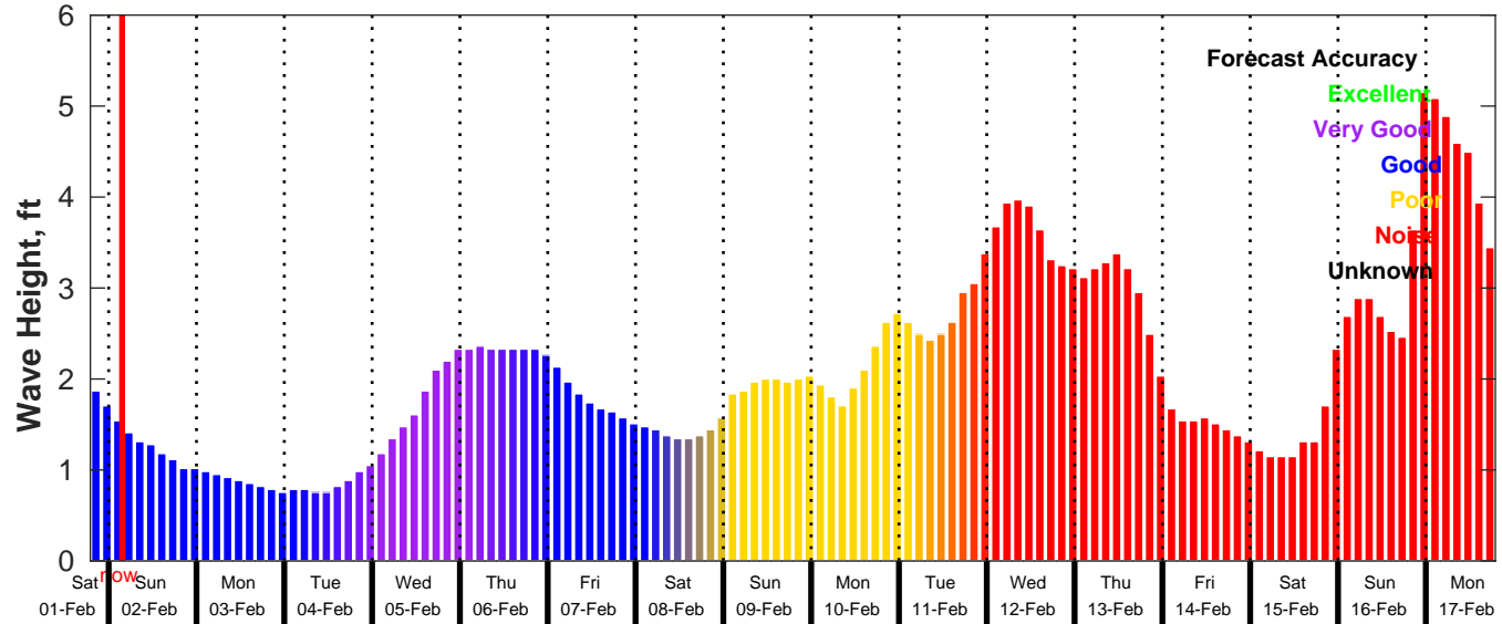
GFS Wave Forecast for NDBC 42084 from 01-Feb-2025 19:00:00 to 17-Feb-2025 19:00:00
