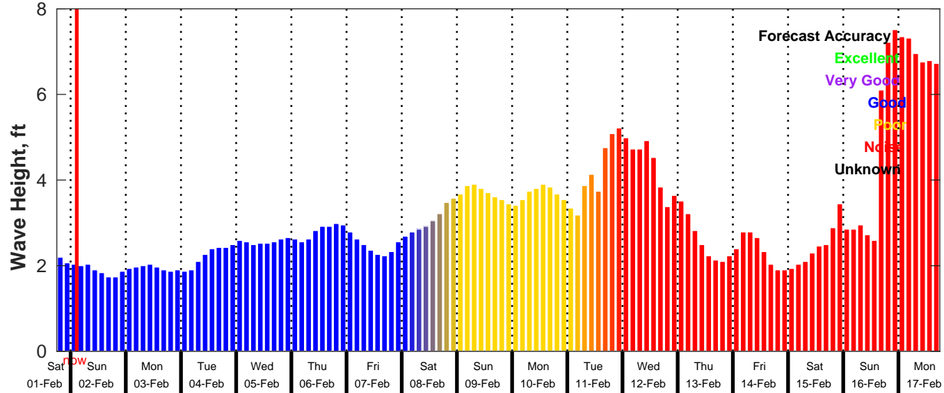
GFS Wave Forecast for NDBC 42092 from 01-Feb-2025 18:00:00 to 17-Feb-2025 18:00:00
