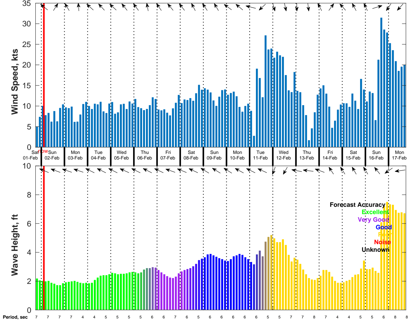
Wind & Wave Forecast for NDBC 42092 from 01-Feb-2025 18:00:00 to 17-Feb-2025 18:00:00
