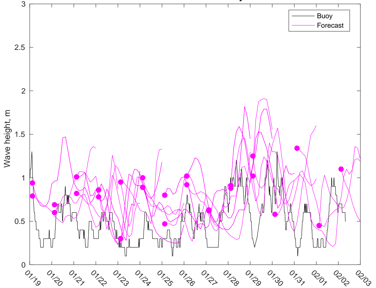
NDBC 44020 vs CMEMSWaves: 7 to 10 day forecast
