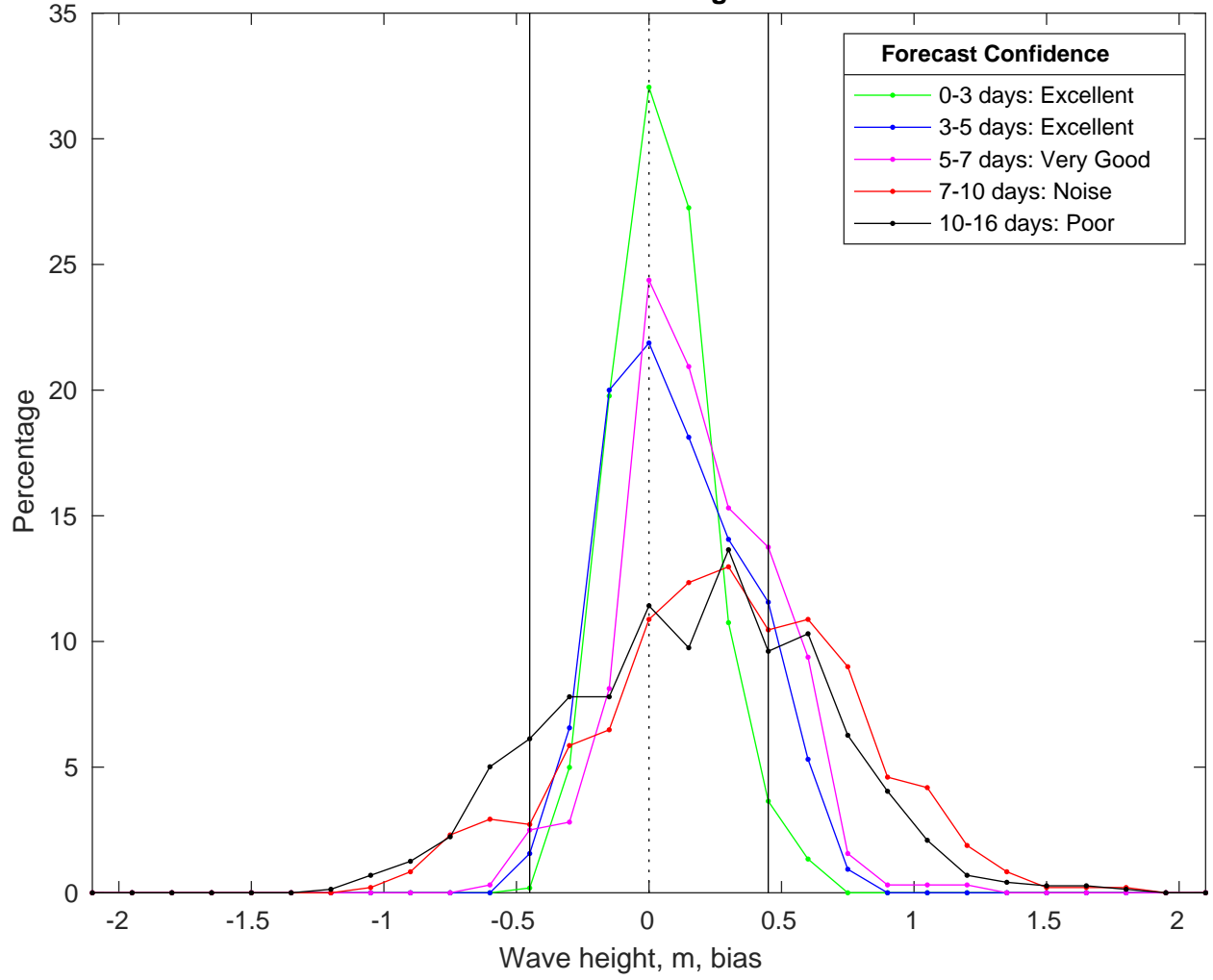
NDBC 44020 vs GFSWaves Bias Histogram: 02-Feb-2025
