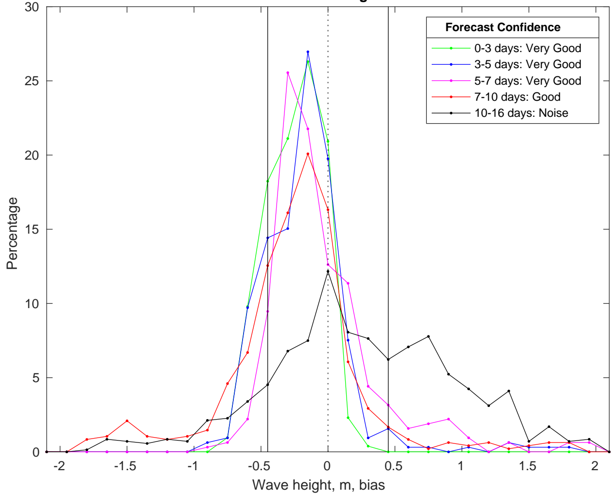
NDBC 46011 vs GFSWaves Bias Histogram: 02-Feb-2025
