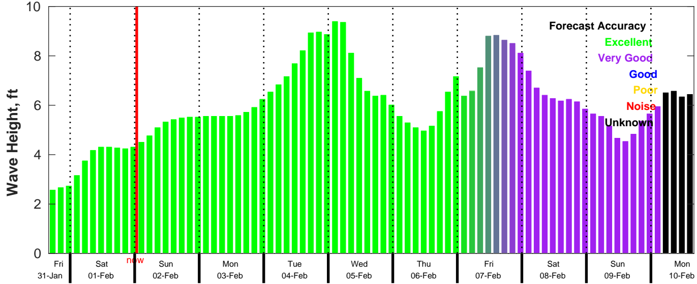
CMEMS Wave Forecast for NDBC 46011 from 31-Jan-2025 16:00:00 to 10-Feb-2025 16:00:00
