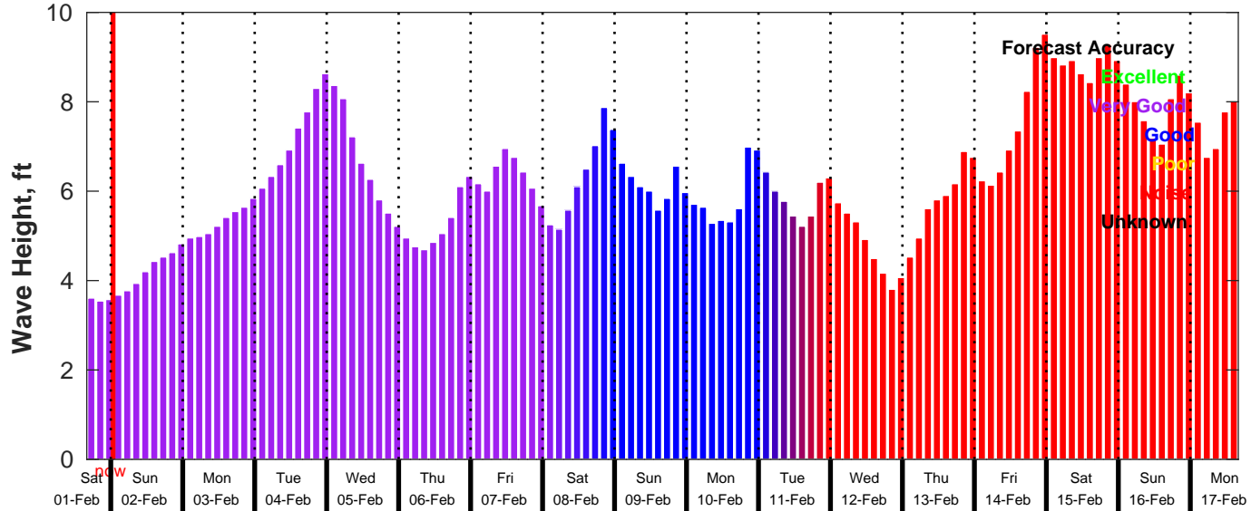
GFS Wave Forecast for NDBC 46011 from 01-Feb-2025 16:00:00 to 17-Feb-2025 16:00:00
