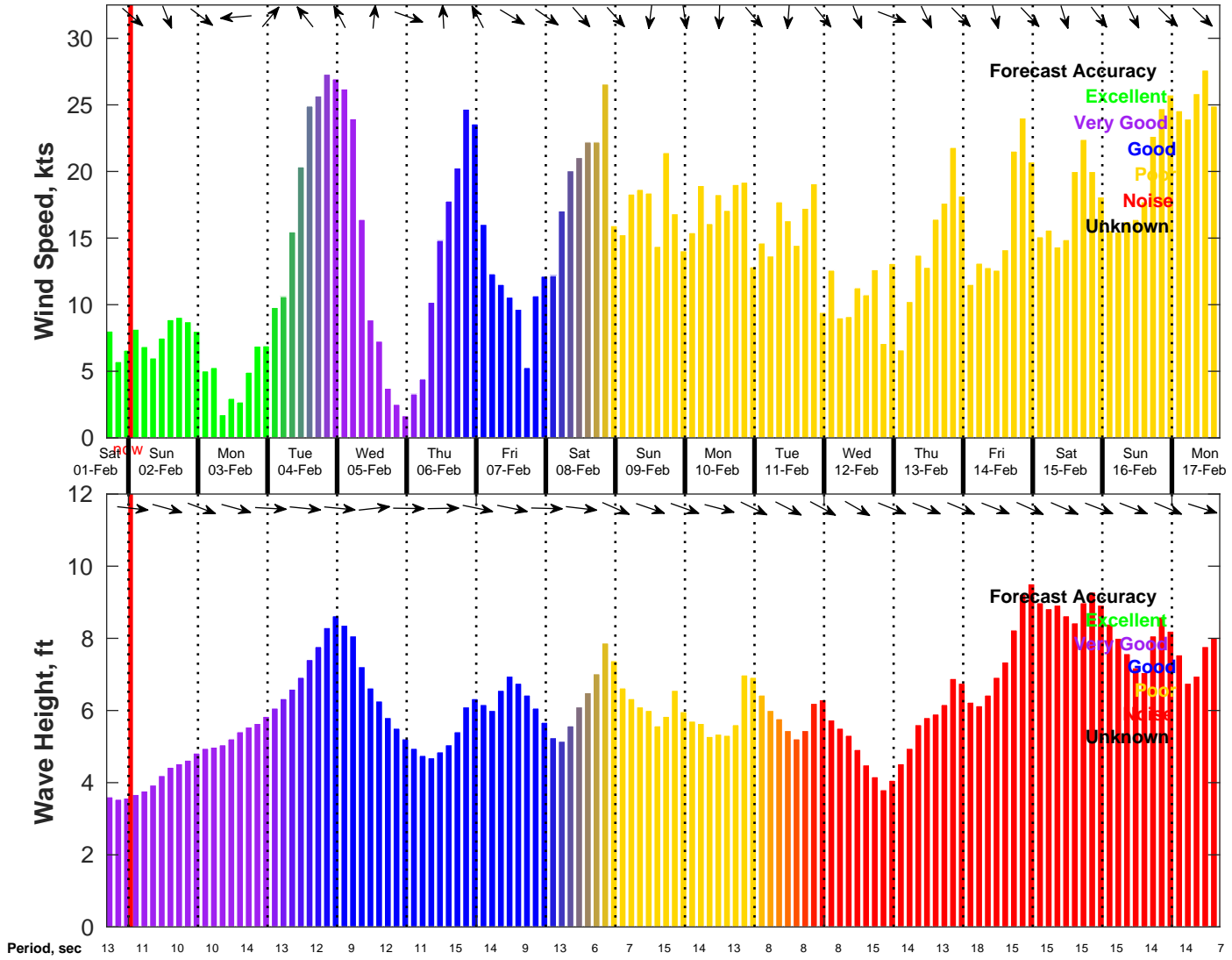
Wind & Wave Forecast for NDBC 46011 from 01-Feb-2025 16:00:00 to 17-Feb-2025 16:00:00
