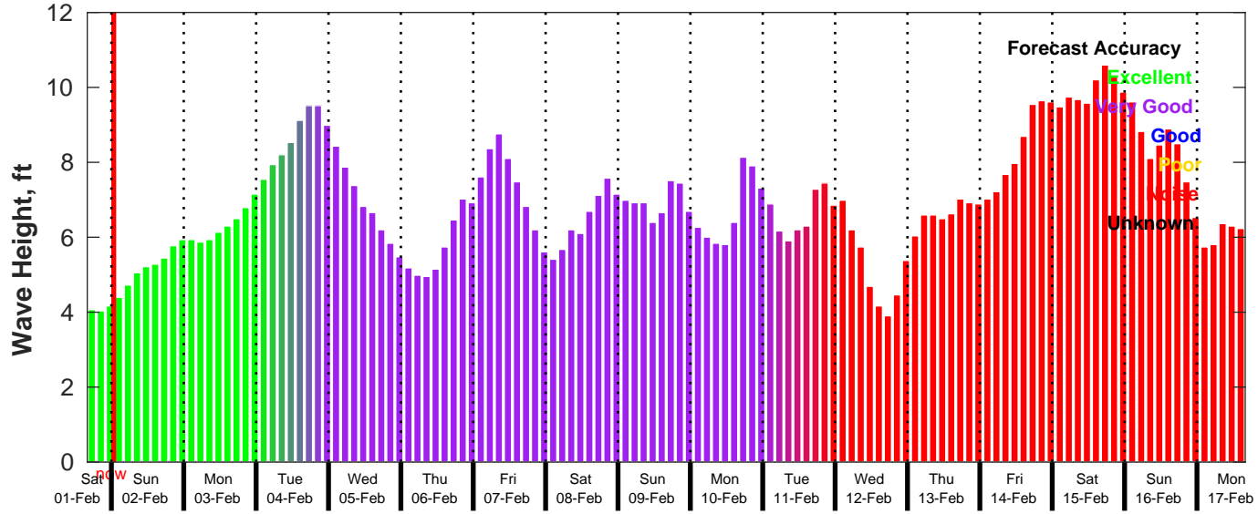
GFS Wave Forecast for NDBC 46028 from 01-Feb-2025 16:00:00 to 17-Feb-2025 16:00:00
