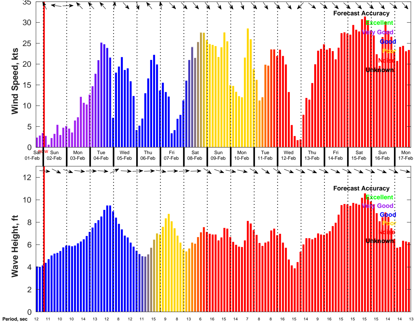
Wind & Wave Forecast for NDBC 46028 from 01-Feb-2025 16:00:00 to 17-Feb-2025 16:00:00
