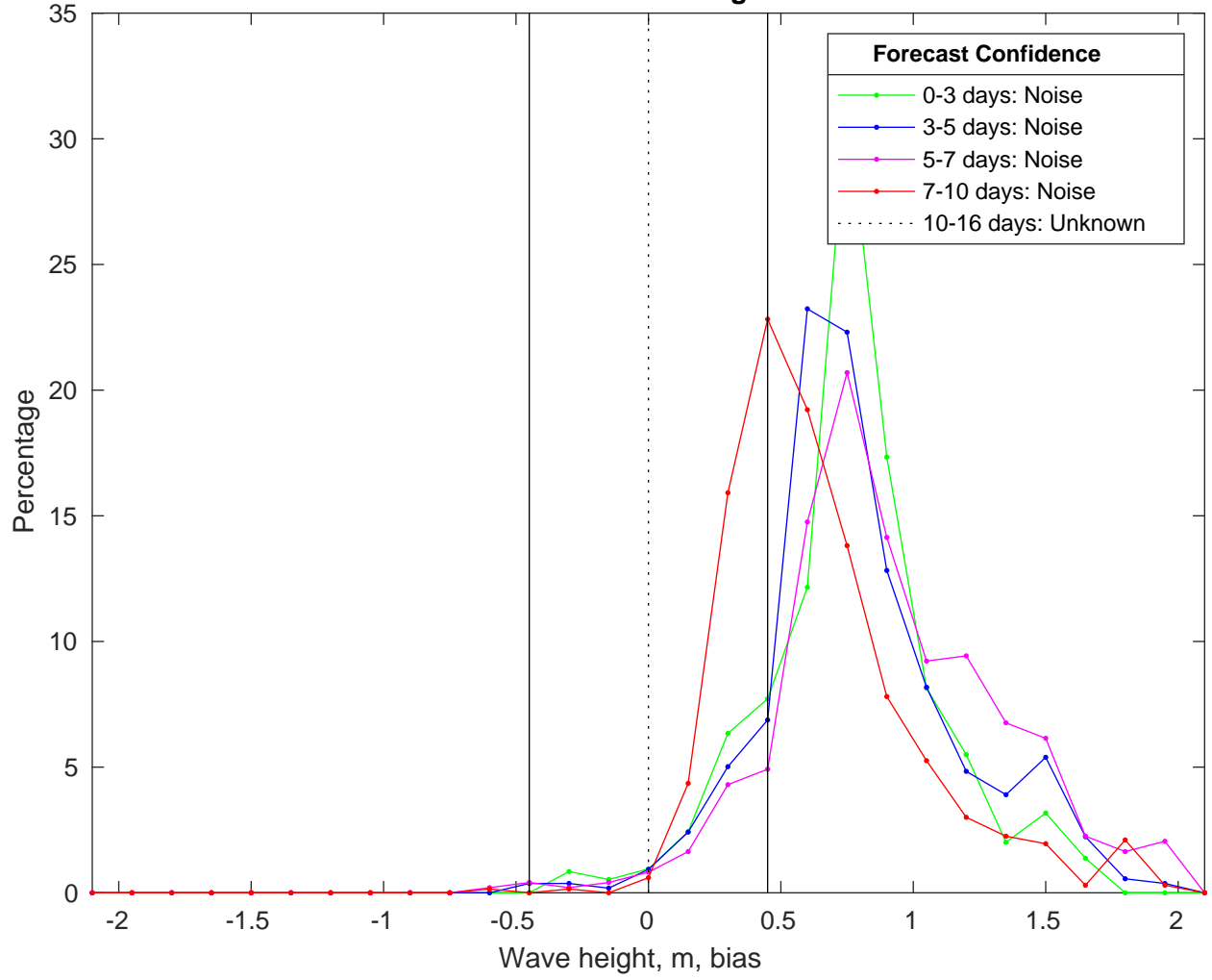
NDBC 46053 vs CEMSWaves Bias Histogram: 02-Feb-2025
