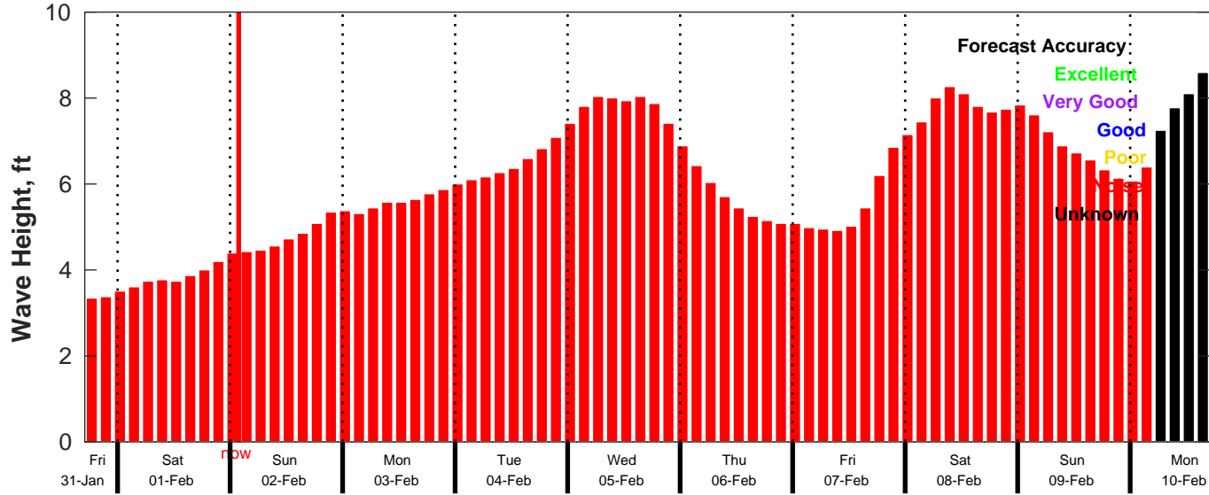
CMEMS Wave Forecast for NDBC 46053 from 31-Jan-2025 17:00:00 to 10-Feb-2025 17:00:00
