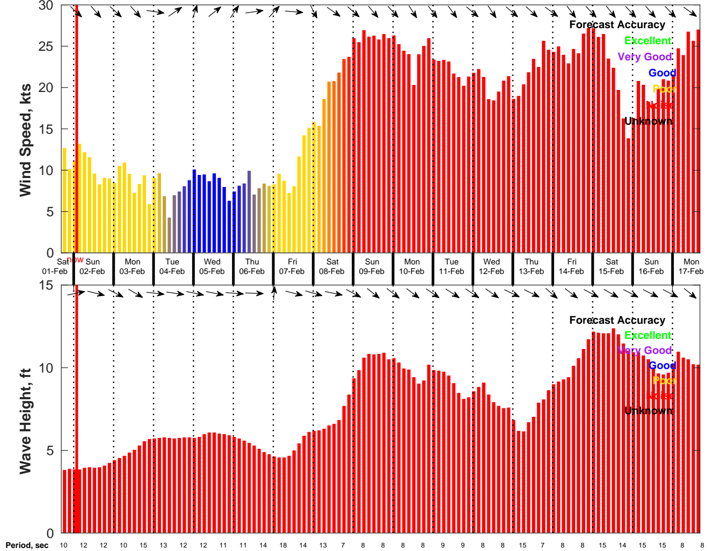
Wind & Wave Forecast for NDBC 46053 from 01-Feb-2025 17:00:00 to 17-Feb-2025 17:00:00
