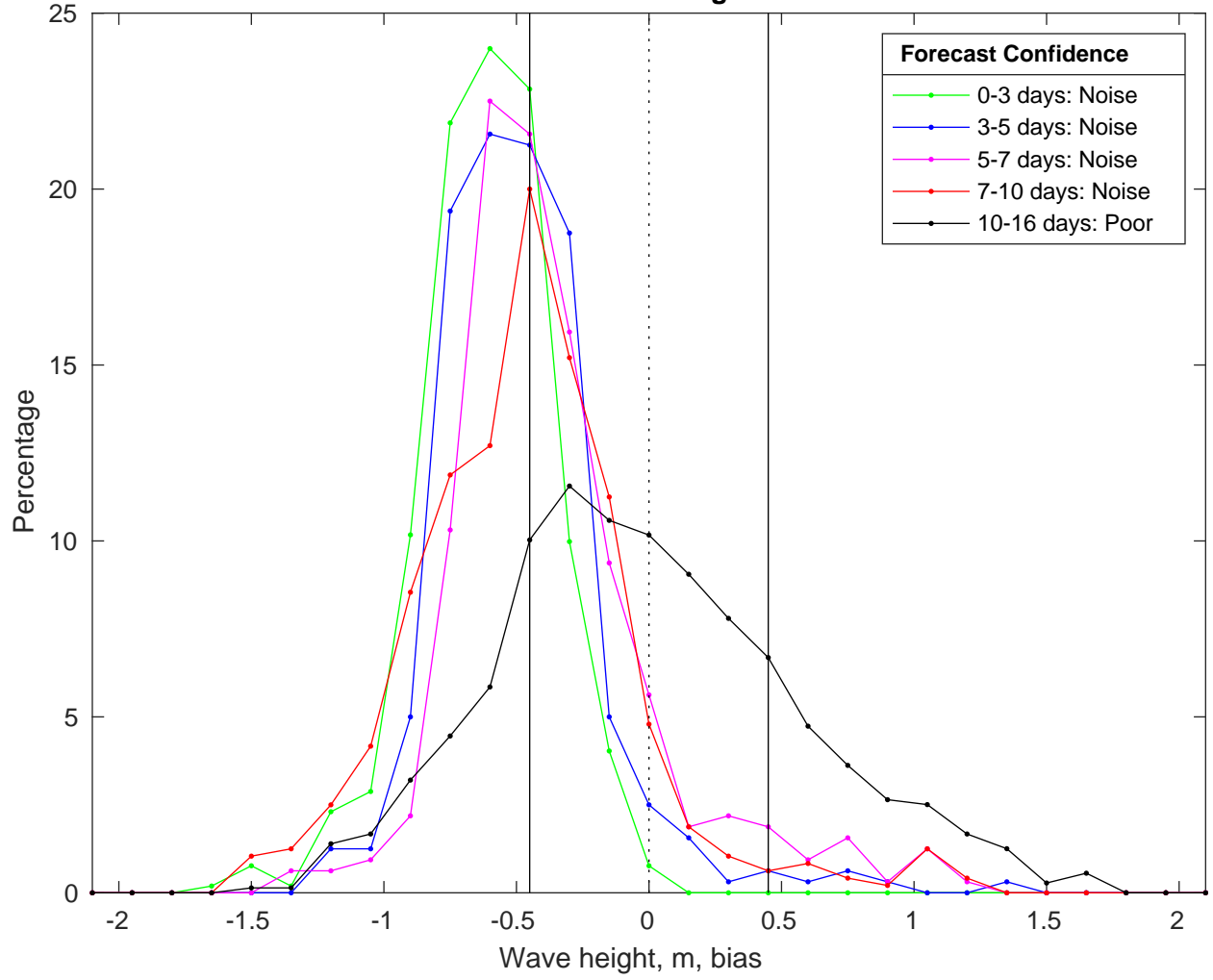
NDBC 46054 vs GFSWaves Bias Histogram: 02-Feb-2025
