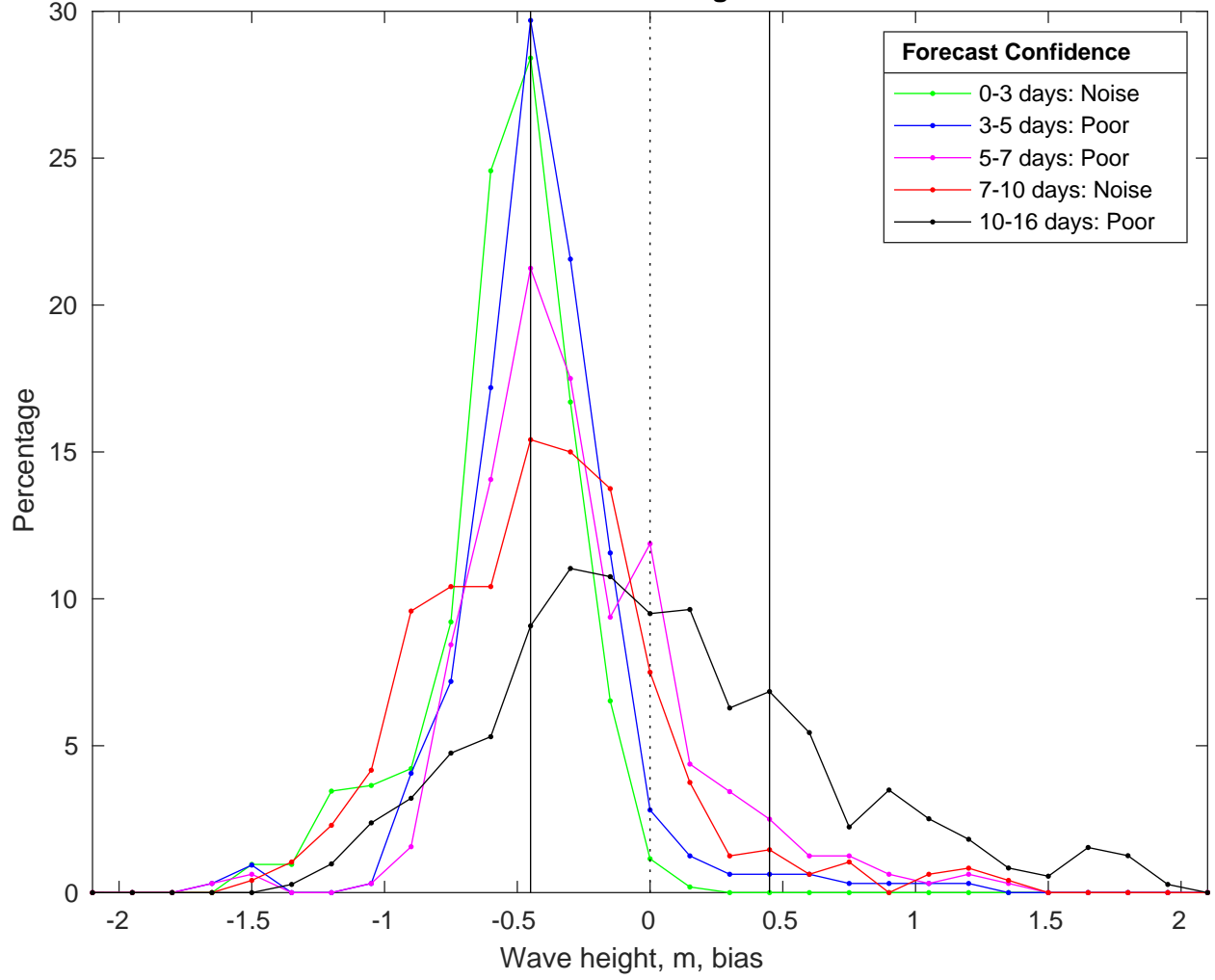
NDBC 46069 vs GFSWaves Bias Histogram: 02-Feb-2025
