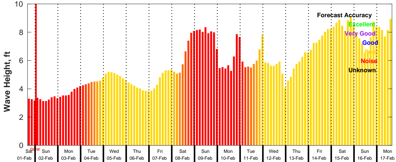
GFS Wave Forecast for NDBC 46069 from 01-Feb-2025 16:00:00 to 17-Feb-2025 16:00:00
