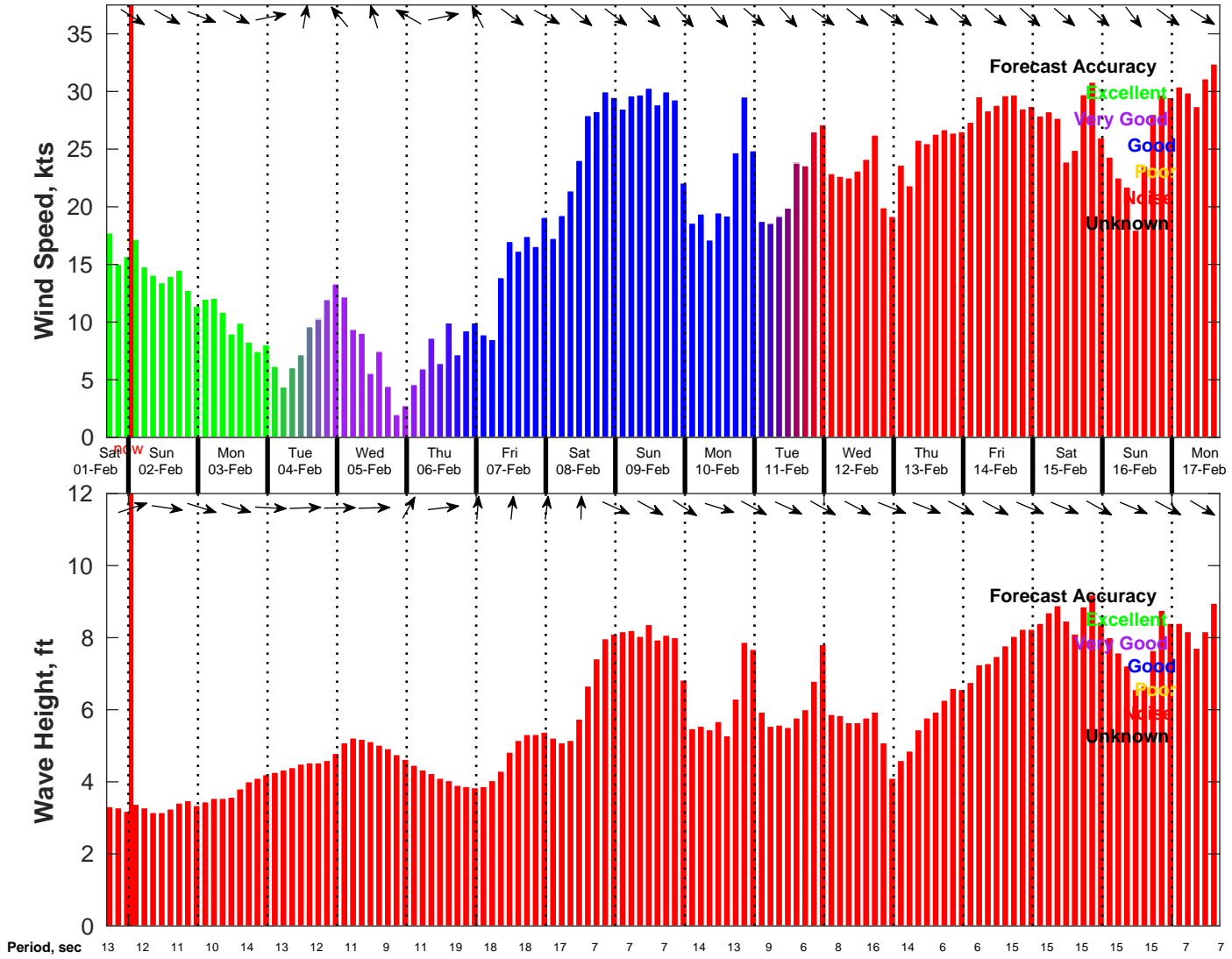
Wind & Wave Forecast for NDBC 46069 from 01-Feb-2025 16:00:00 to 17-Feb-2025 16:00:00
