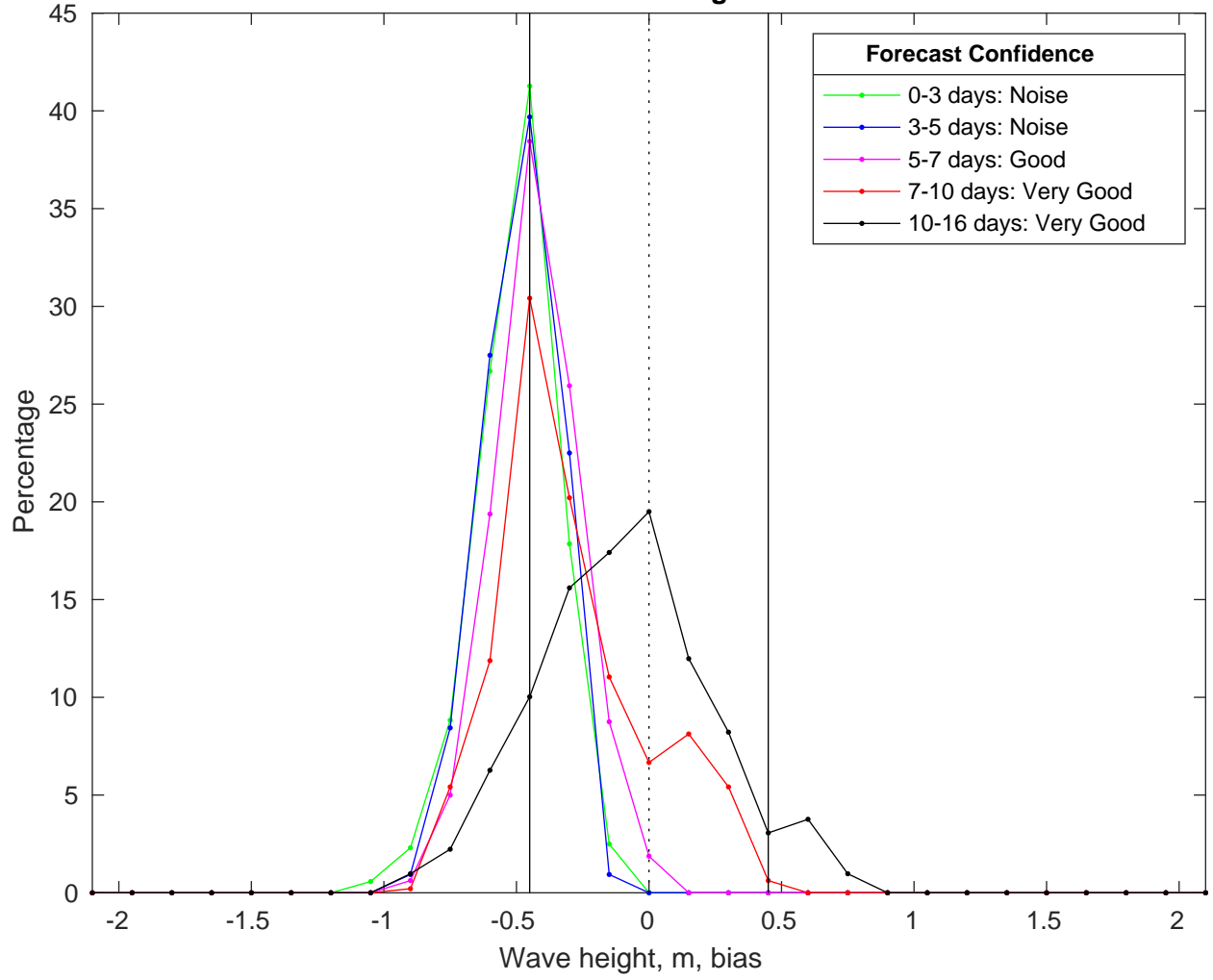
NDBC 51209 vs GFSWaves Bias Histogram: 02-Feb-2025
