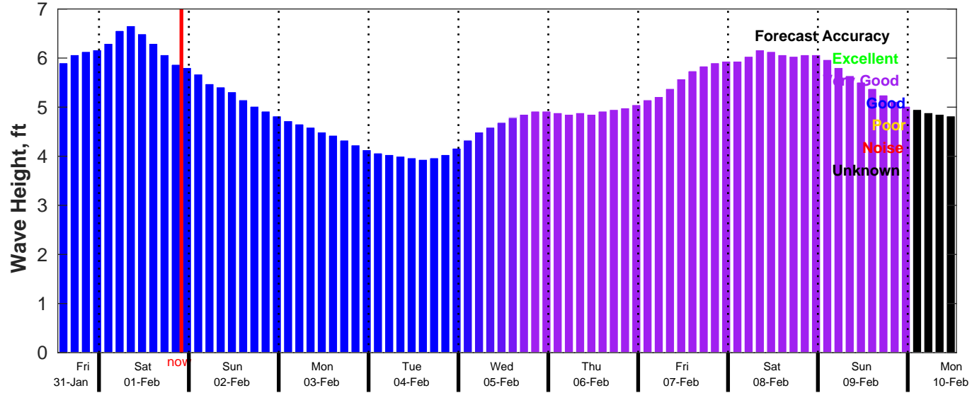
CMEMS Wave Forecast for NDBC 51209 from 31-Jan-2025 13:00:00 to 10-Feb-2025 13:00:00
