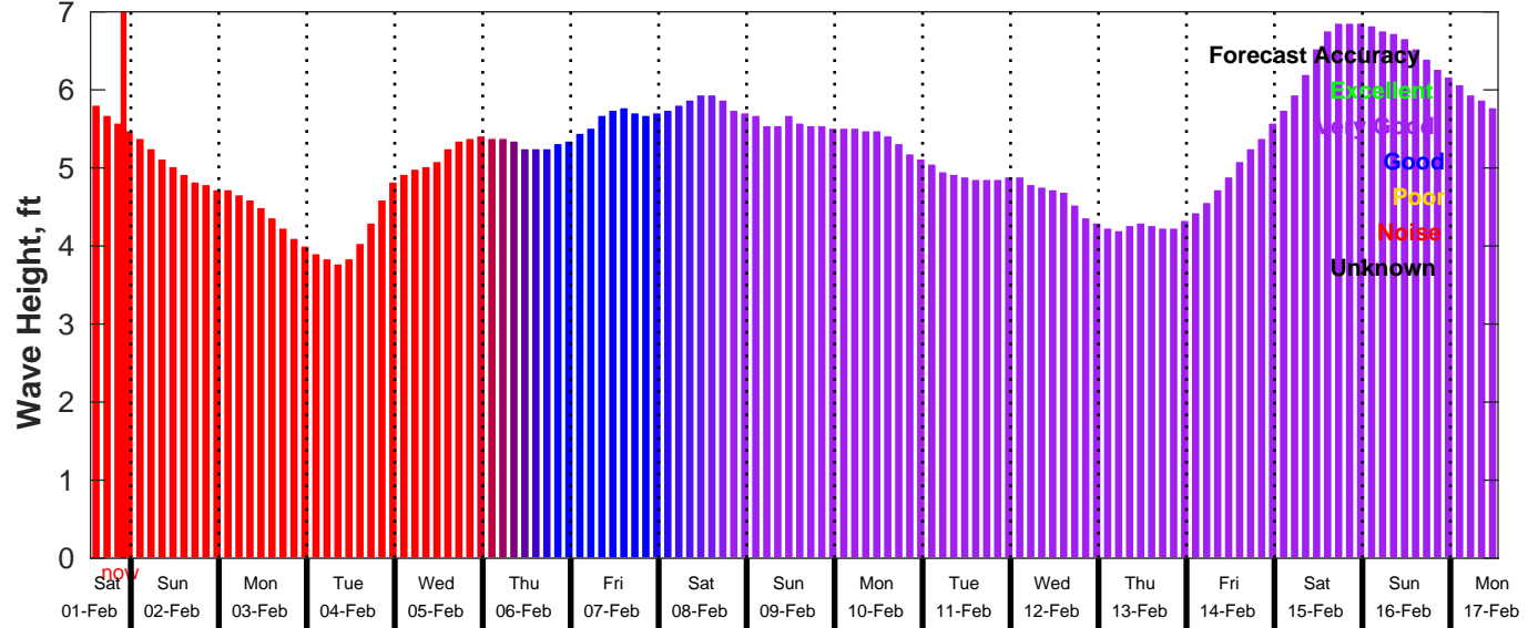
GFS Wave Forecast for NDBC 51209 from 01-Feb-2025 13:00:00 to 17-Feb-2025 13:00:00
