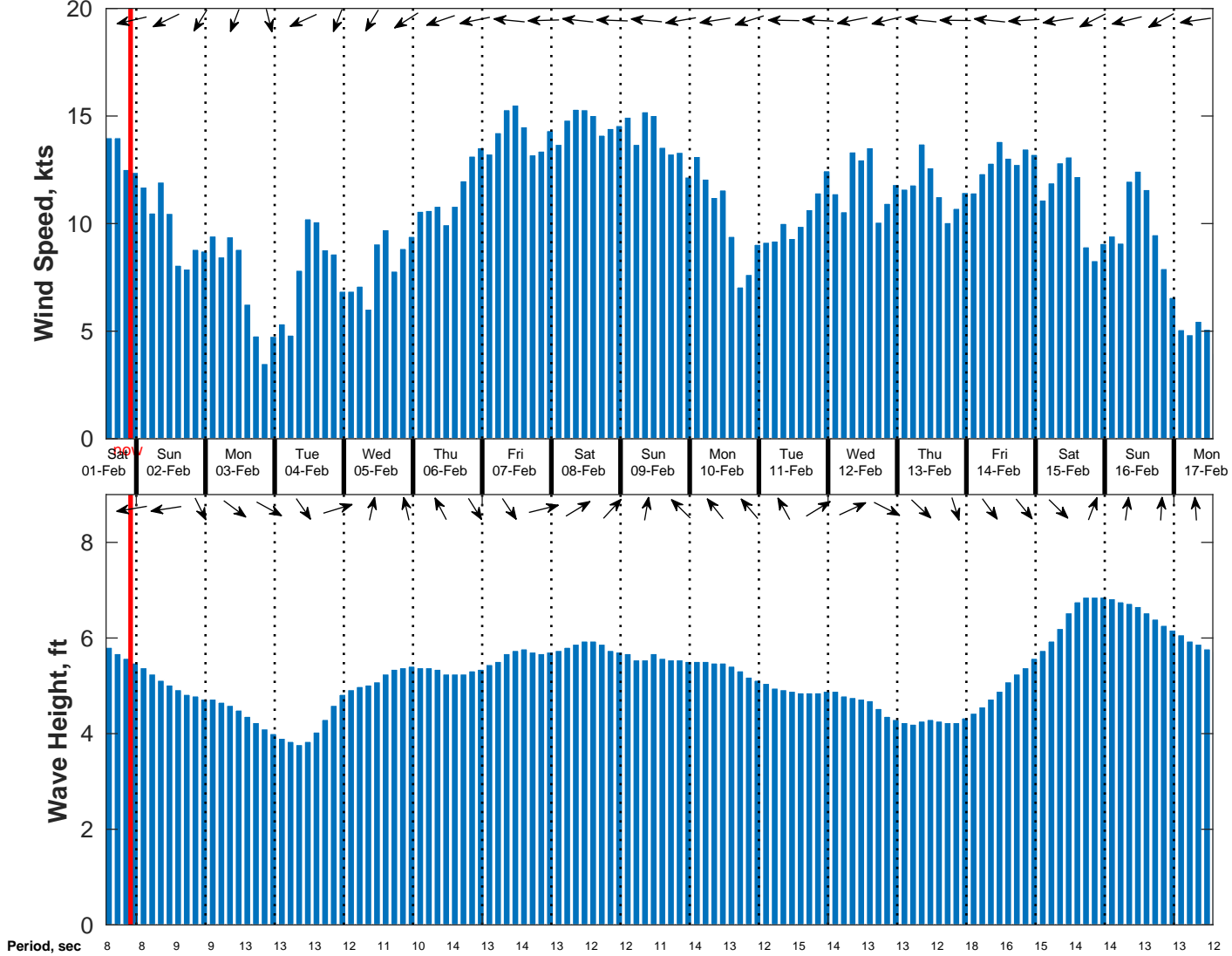
Wind & Wave Forecast for NDBC 51209 from 01-Feb-2025 13:00:00 to 17-Feb-2025 13:00:00
