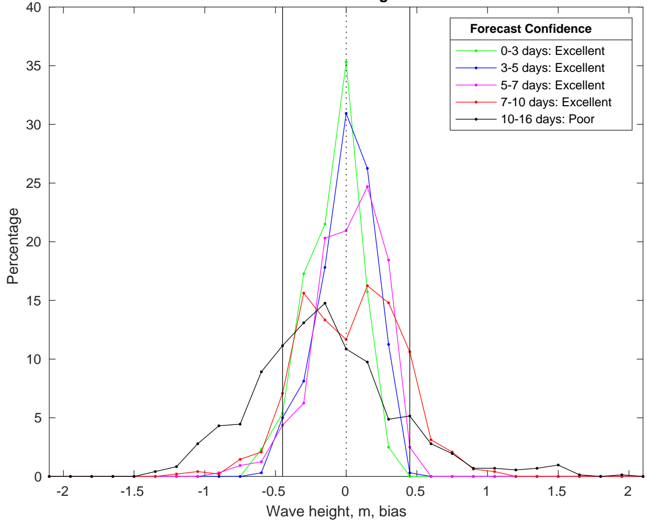
NDBC 52211 vs GFSWaves Bias Histogram: 02-Feb-2025
