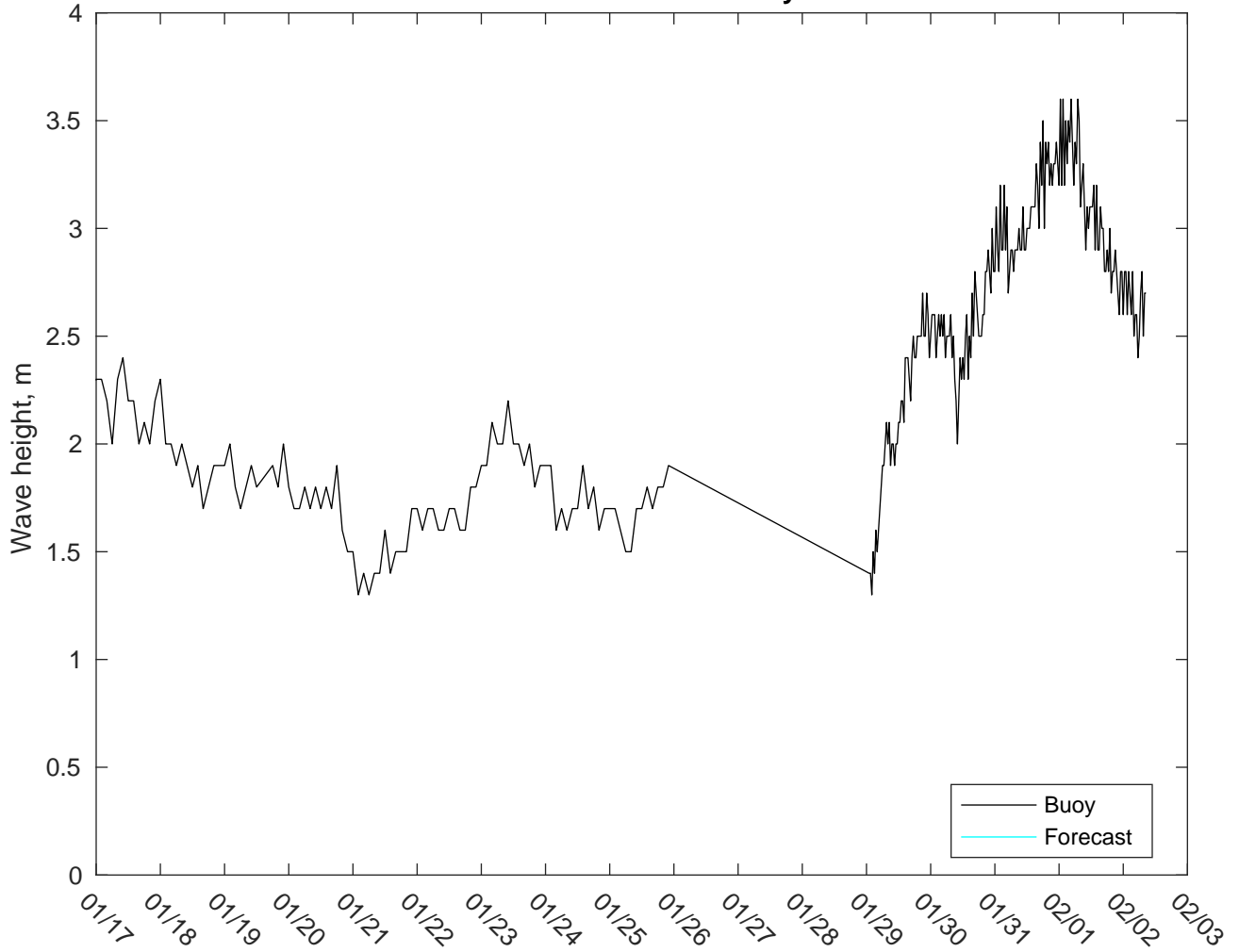
NDBC 52212 vs CMEMSWaves: 5 to 7 day forecast
