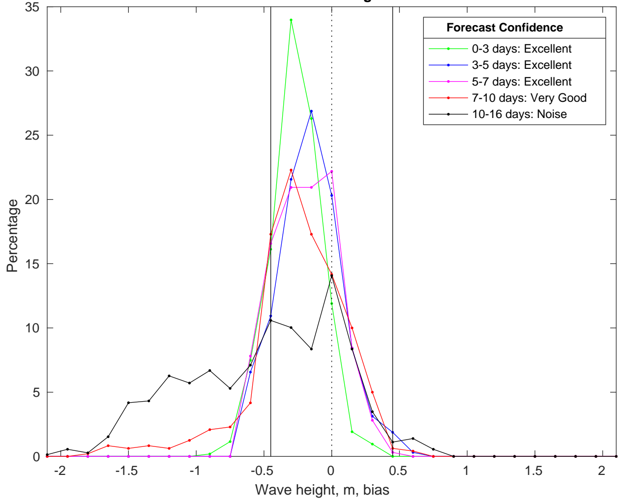
NDBC 52212 vs GFSWaves Bias Histogram: 02-Feb-2025
