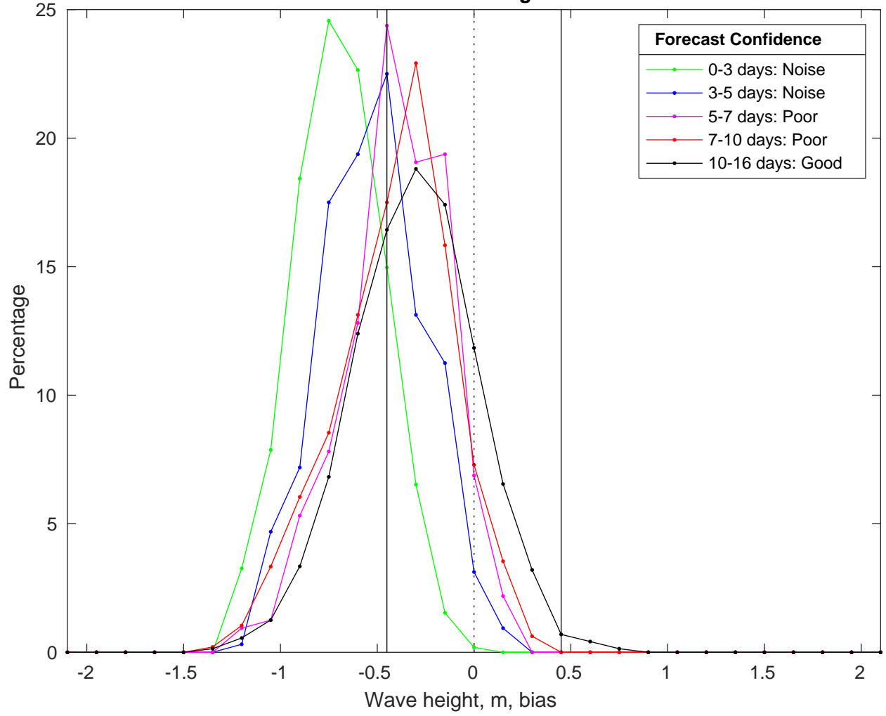
NDBC 52213 vs GFSWaves Bias Histogram: 02-Feb-2025
