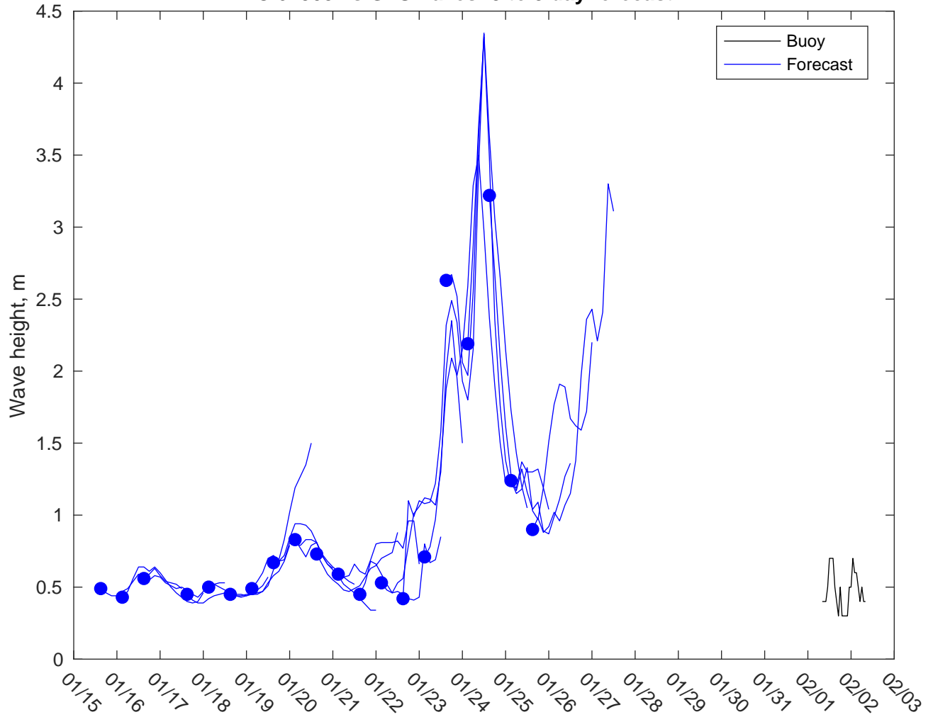
NDBC 62305 vs GFSWaves: 3 to 5 day forecast
