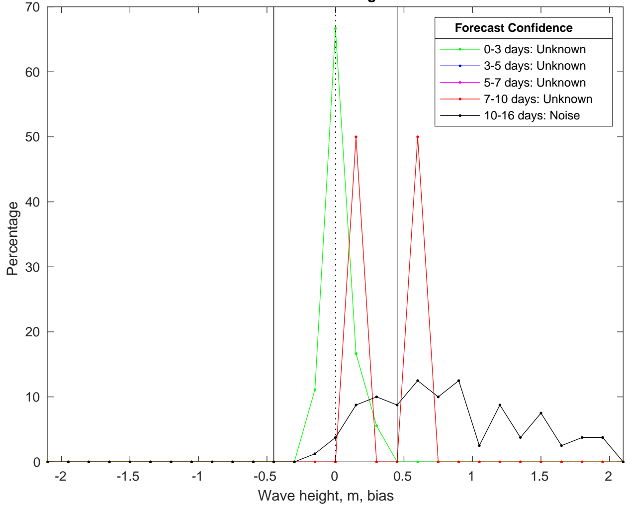
NDBC 62305 vs GFSWaves Bias Histogram: 02-Feb-2025
