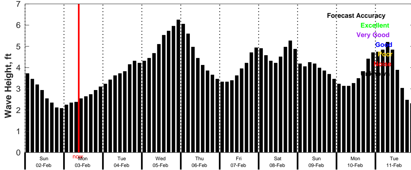
CMEMS Wave Forecast for NDBC 62305 from 01-Feb-2025 00:00:00 to 11-Feb-2025 00:00:00
