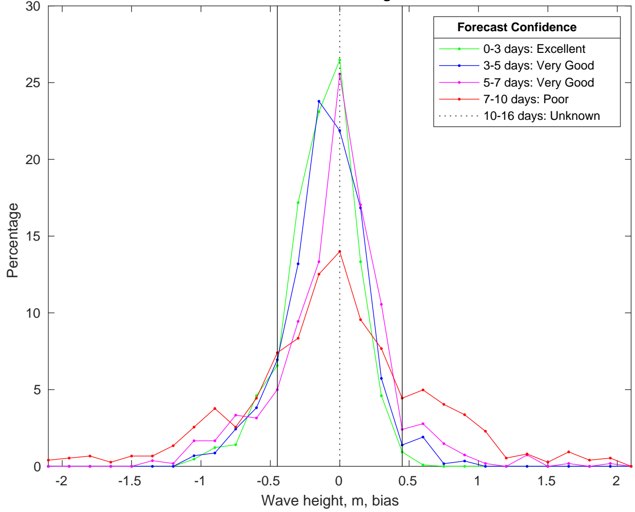
NDBC 41004 vs CMEMSWaves Bias Histogram: 03-Feb-2025
