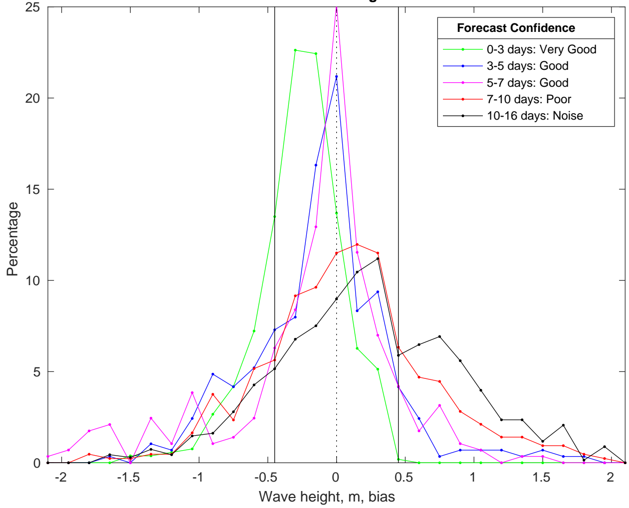
NDBC 41004 vs GFSWaves Bias Histogram: 03-Feb-2025
