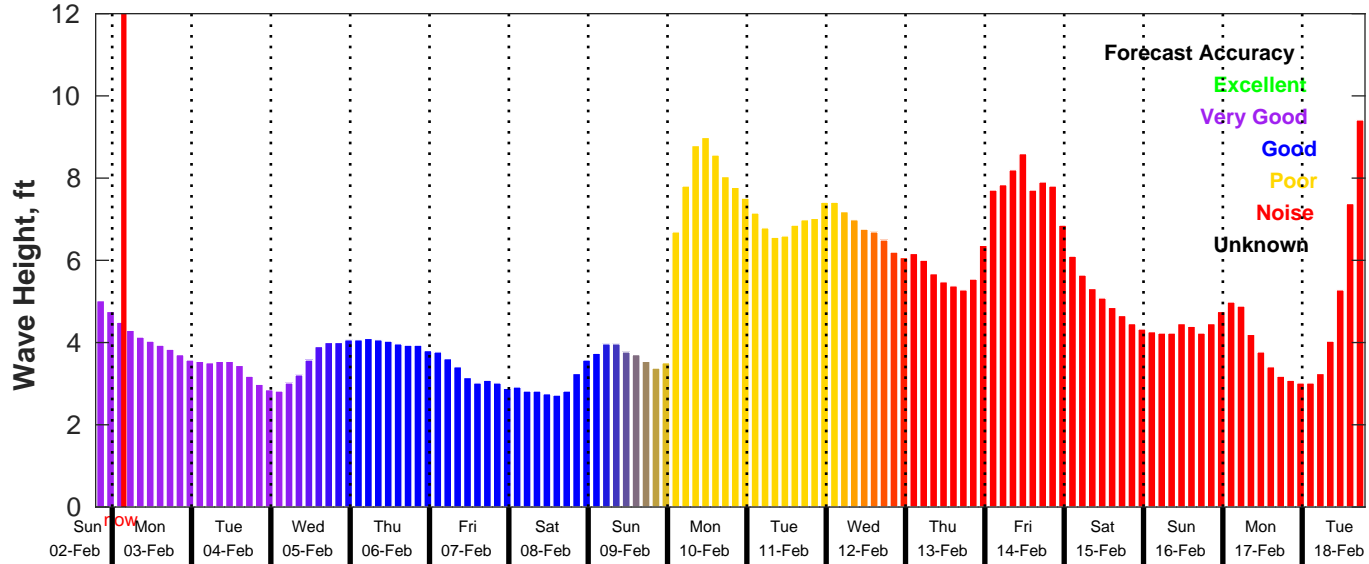
GFS Wave Forecast for NDBC 41004 from 02-Feb-2025 19:00:00 to 18-Feb-2025 19:00:00
