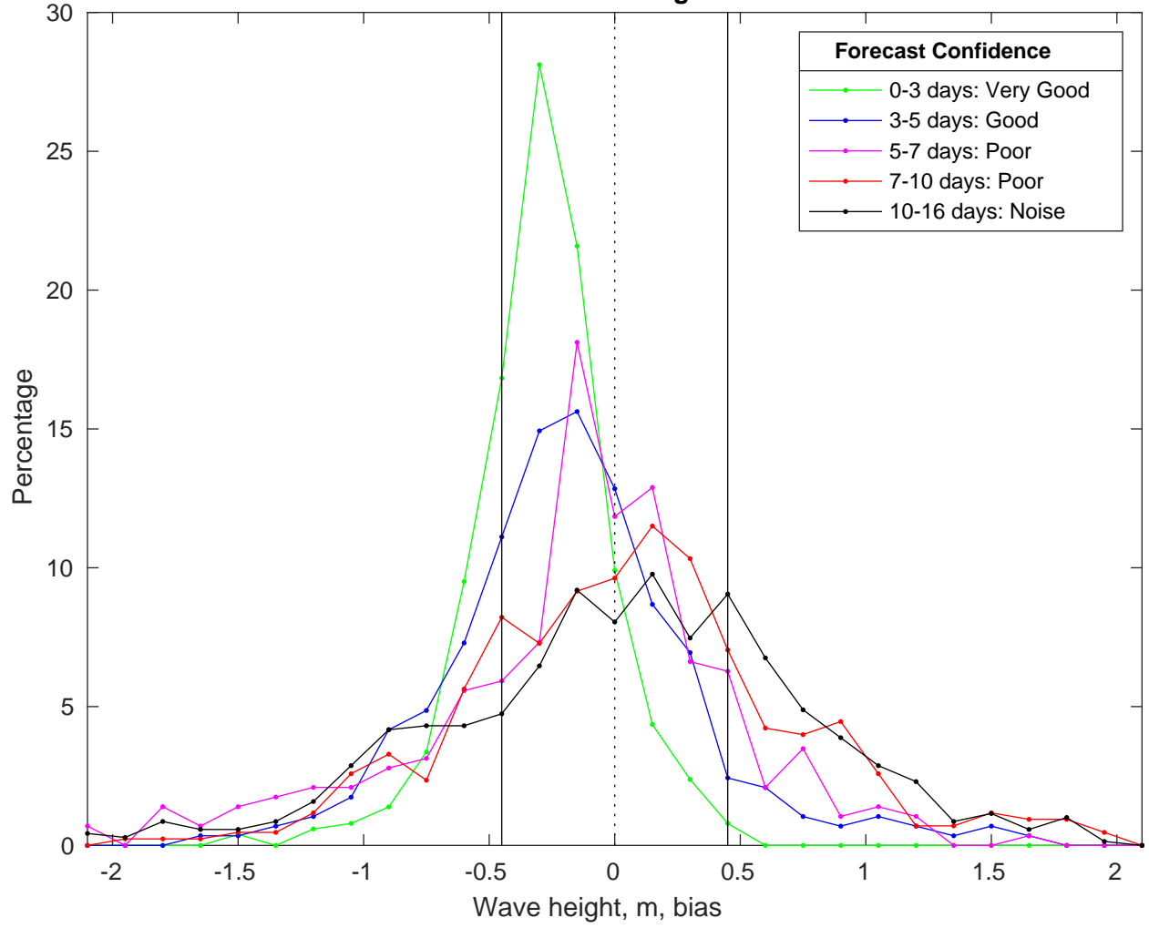
NDBC 41013 vs GFSWaves Bias Histogram: 03-Feb-2025
