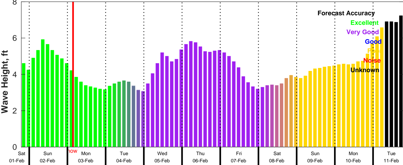
CMEMS Wave Forecast for NDBC 41013 from 01-Feb-2025 19:00:00 to 11-Feb-2025 19:00:00
