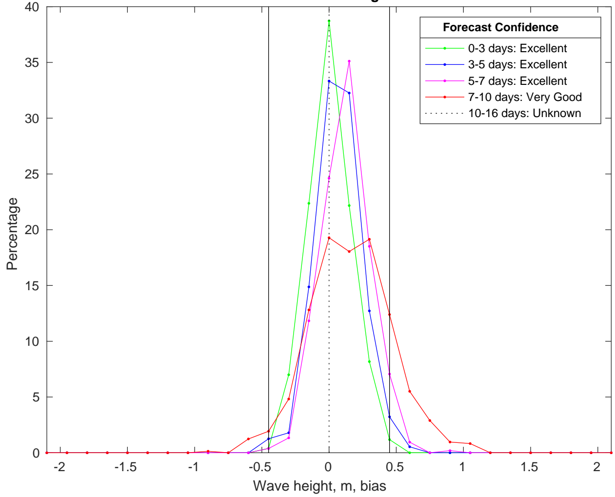
NDBC 41040 vs CMEMSWaves Bias Histogram: 03-Feb-2025
