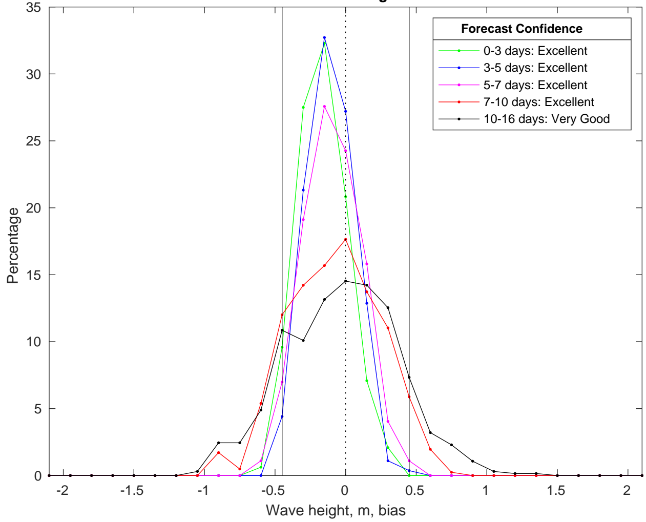
NDBC 41040 vs GFSWaves Bias Histogram: 03-Feb-2025
