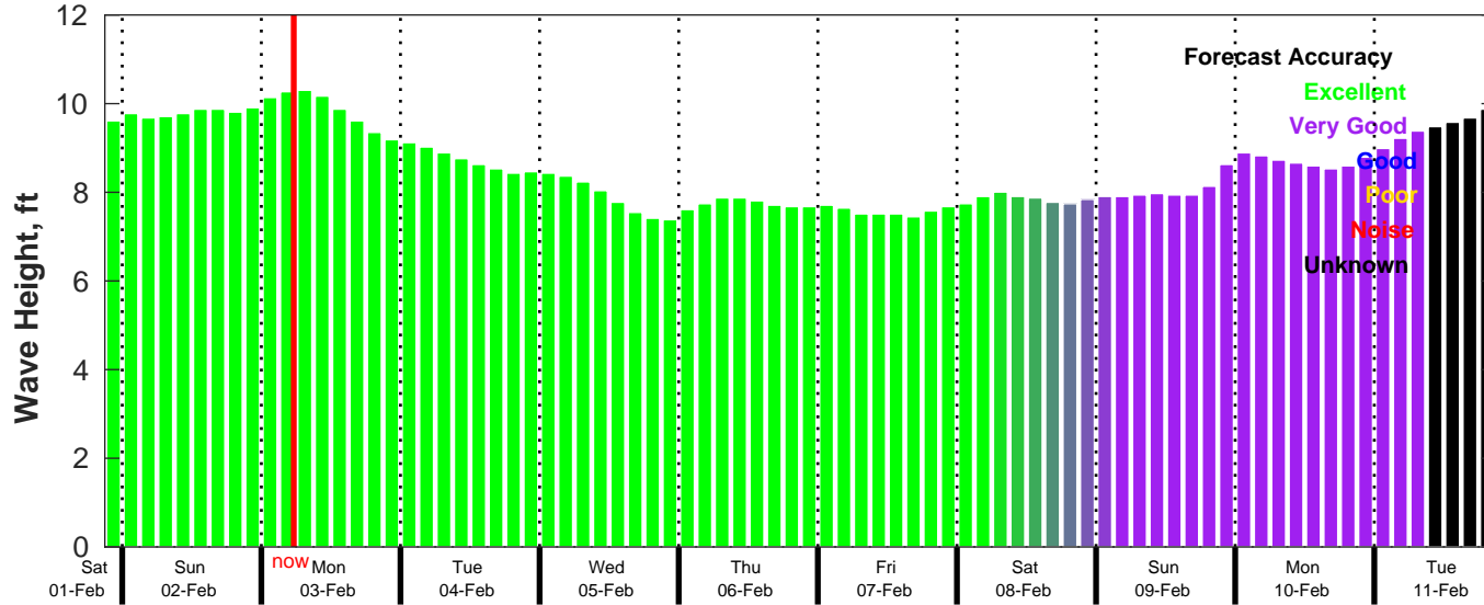
CMEMS Wave Forecast for NDBC 41040 from 01-Feb-2025 21:00:00 to 11-Feb-2025 21:00:00
