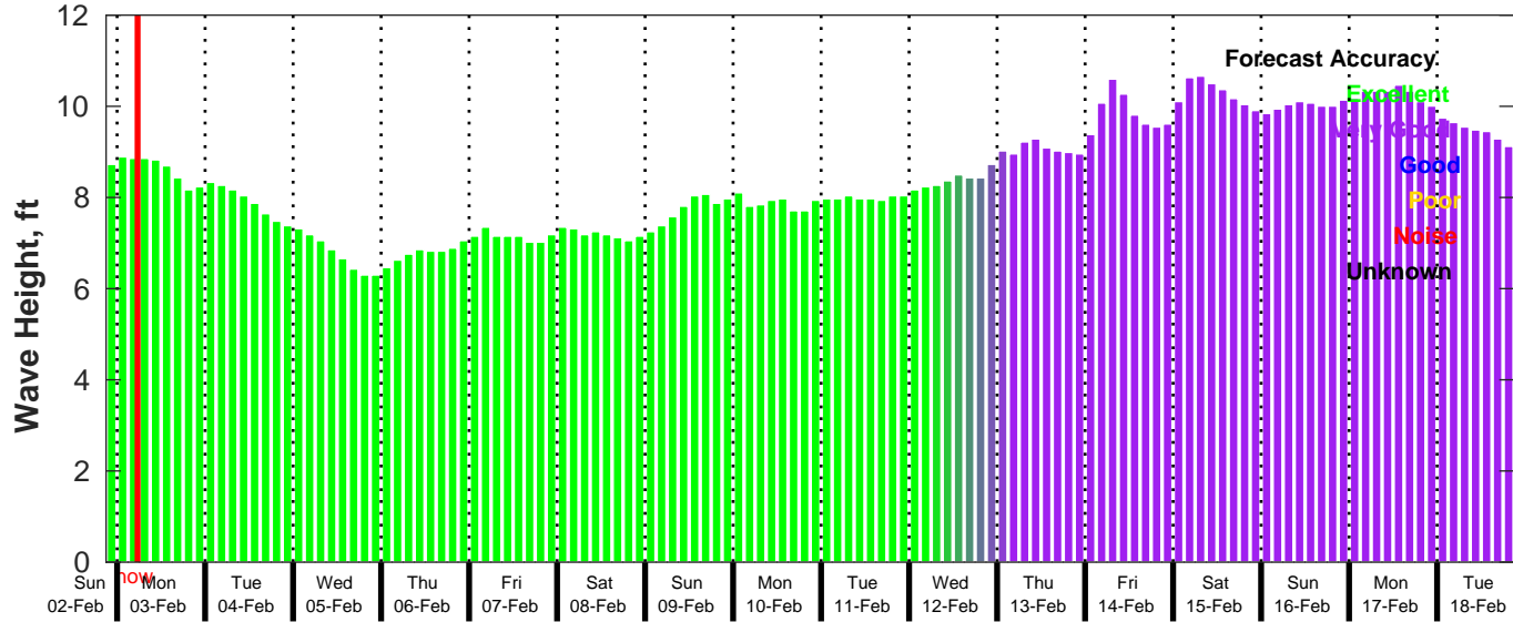
GFS Wave Forecast for NDBC 41040 from 02-Feb-2025 21:00:00 to 18-Feb-2025 21:00:00
