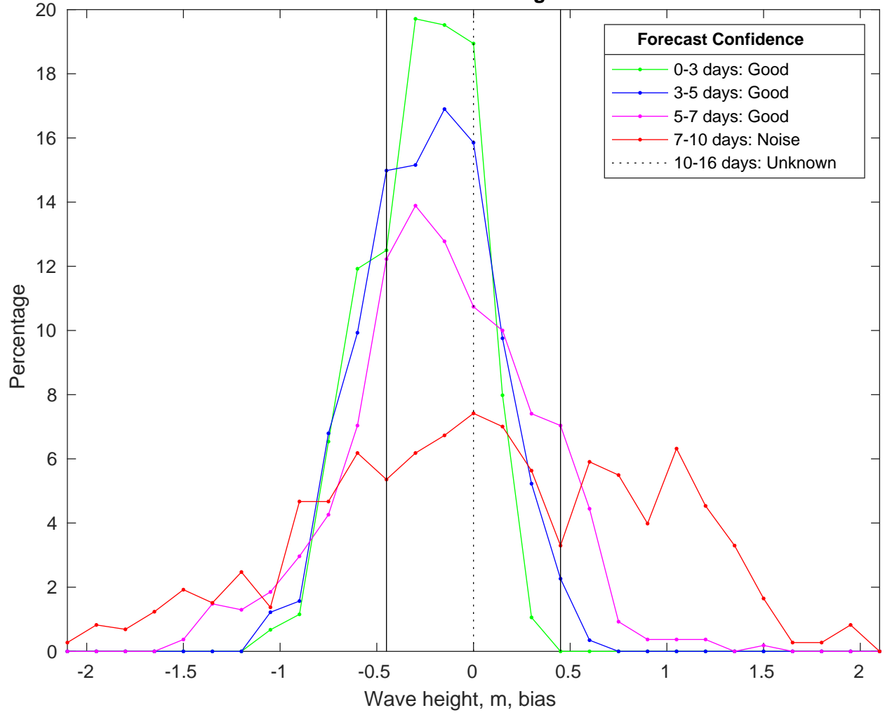
NDBC 42019 vs CMEMSWaves Bias Histogram: 03-Feb-2025
