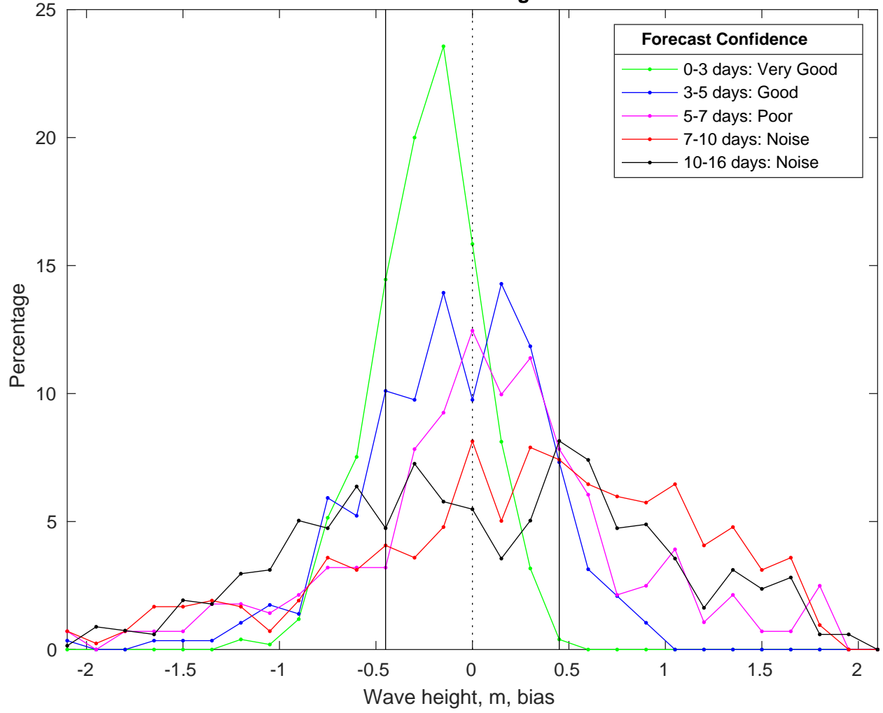
NDBC 42019 vs GFSWaves Bias Histogram: 03-Feb-2025
